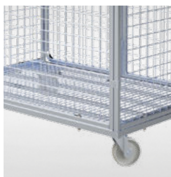
CHASSIS MADE OF RECTANGULAR TUBE 30 X 20 MM
